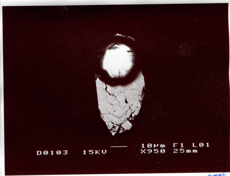
95-34, Grain #24, Cp 45 788
