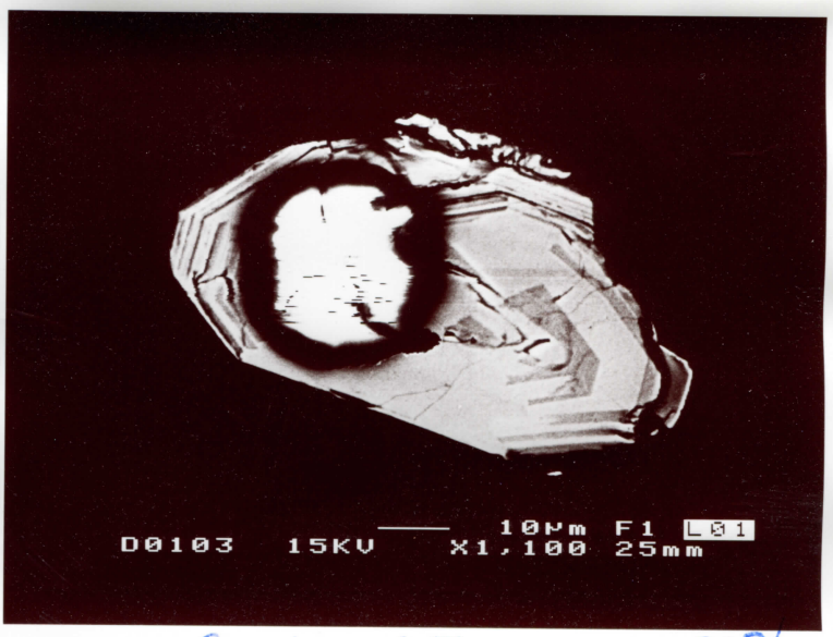
95-34, Grain #12, BSE 807
