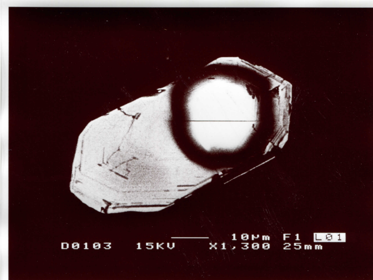
95-34, BSE #25
