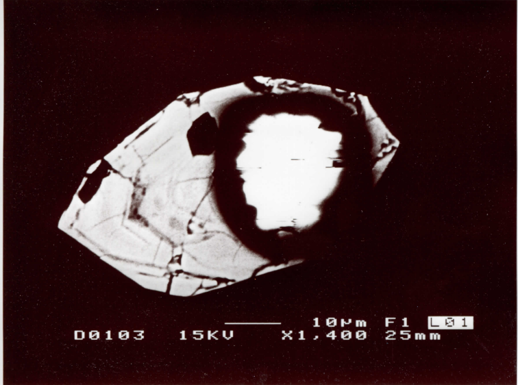
95-34, Grain #20, BSE 809
