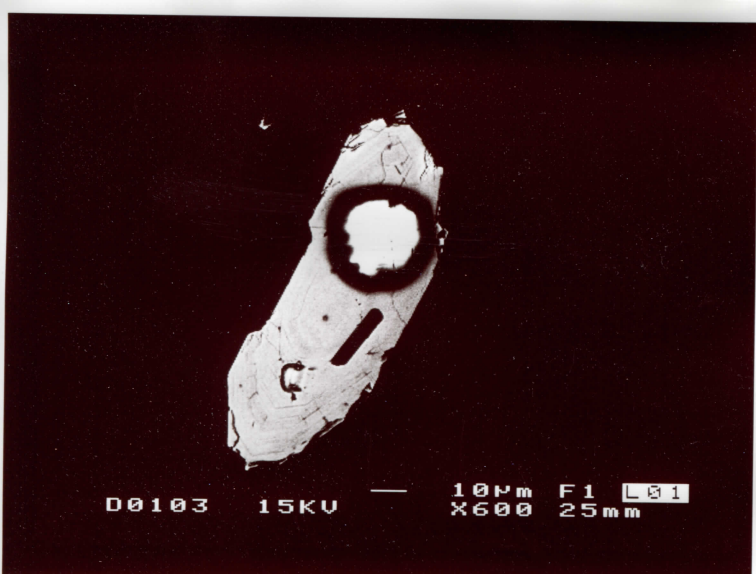
95-34, Grain #10, BSE 803
