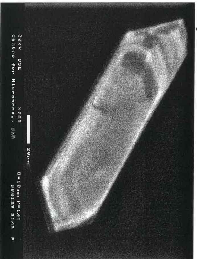
Cathodoluminescence image
