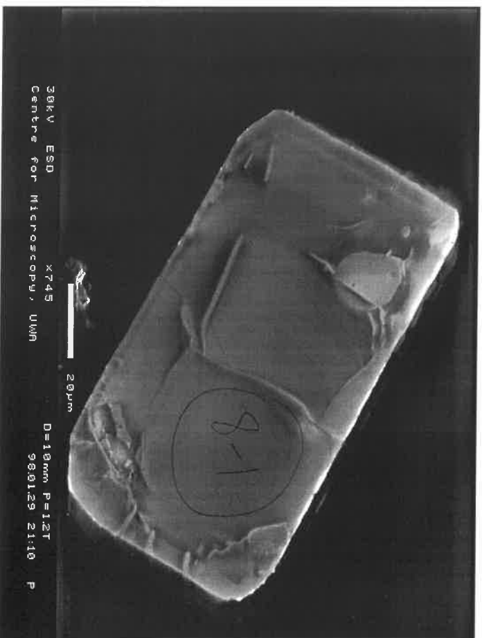
Secondary electron (Charge Contrast) image File: 9749c08s
