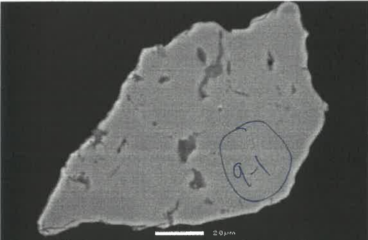
30kV BSE X840 D=12mm P=1.2T Centre for Microscopy, UWA 98.12.02 01:05 P 9884b09b.tif
