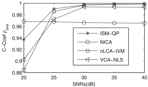
Fig. 4. \rho_{ave} of different algorithms versus SNRs, where the percentage of corrupted pixels is 25%.
