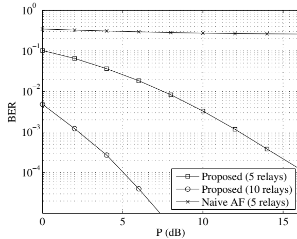
Fig. 4: Example 2: BER versus P for different L .
