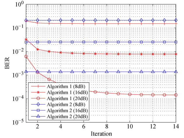
Fig. 3. Example 1: BER versus the number of iterations, K = 2 .
