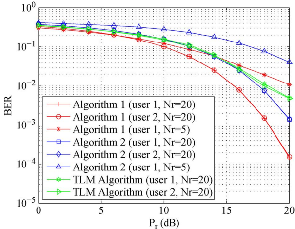
Fig. 5. Example 2: BER versus P_r for each transmitter-receiver pair, K = 2 .
