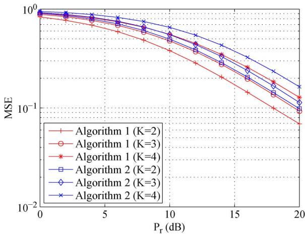
Fig. 6. Example 3: MSE versus P_r for different K .
