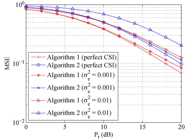
Fig. 7. Example 4: Effect of CSI mismatch on the proposed algorithms.
