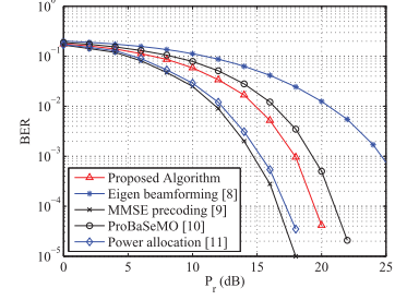
Fig. 2. Example 1: BER of five algorithms versus P_r .
