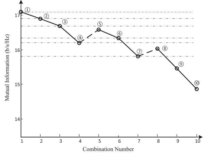
Fig. 2. Sum MI at all subchannel allocation schemes. N_s = 3 , N_r = 5 , N_d = 5 , N_1 = 3 , N_2 = 2 , and \text{SNR}_s = \text{SNR}_r = 20 dB.
