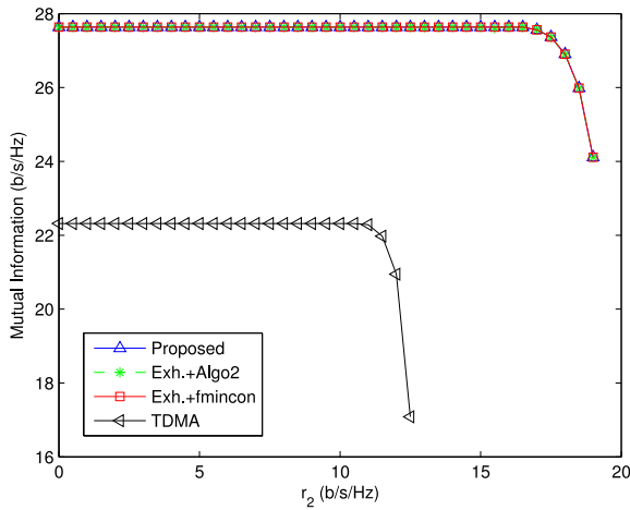
Fig. 14. Example 5: MI versus r_2 with fixed \mathbf{H} and \mathbf{G} . N_s = 8 , N_r = 10 , N_d = 10 , N_1 = 5 , N_2 = 3 , d = 1 , r_1 = 0.5 b/s/Hz, and \text{SNR}_s = \text{SNR}_r = 20 dB.
