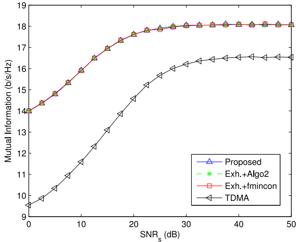
Fig. 7. Example 2: MI versus \text{SNR}_s . N_s = 3 , N_r = 5 , N_d = 5 , N_1 = 3 , N_2 = 2 , d = 1 , r_1 = r_2 = 0.5 b/s/Hz, and \text{SNR}_r = 20 dB.
