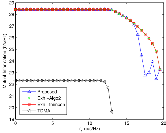
Fig. 13. Example 5: MI versus r_1 with fixed \mathbf{H} and \mathbf{G} . N_s = 8 , N_r = 10 , N_d = 10 , N_1 = 5 , N_2 = 3 , d = 1 , r_2 = 0.5 b/s/Hz, and \text{SNR}_s = \text{SNR}_r = 20 dB.
