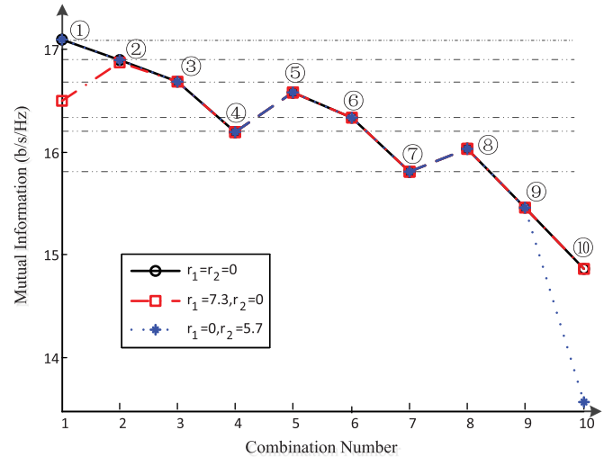
Fig. 4. The impact of QoS constraints on the subchannel allocation schemes. N_s = 3, N_r = 5, N_d = 5, N_1 = 3, N_2 = 2 , and \text{SNR}_s = \text{SNR}_r = 20 dB.
