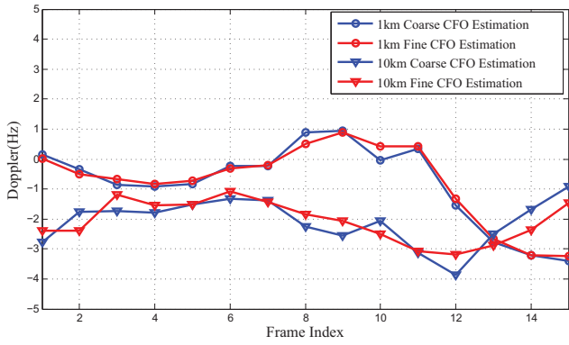
Fig. 11. CFO estimation results at 1km and 10km
