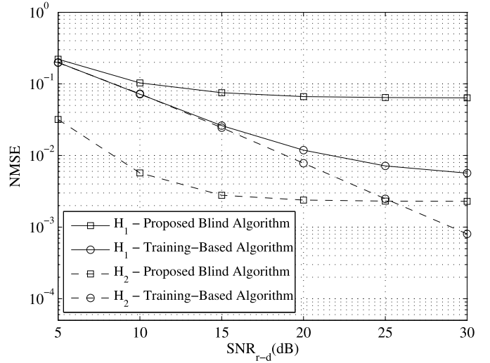
Fig. 6. Example 4: normalized MSE versus \text{SNR}_{r-d} for n_s = n_r = 2 and n_D = 4 with \text{SNR}_{s-r} = 20 dB.
