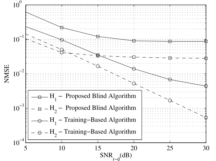
Fig. 7. Example 4: normalized MSE versus \text{SNR}_{r-d} for n_s = n_r = 3 and n_D = 4 with \text{SNR}_{s-r} = 20 dB.
