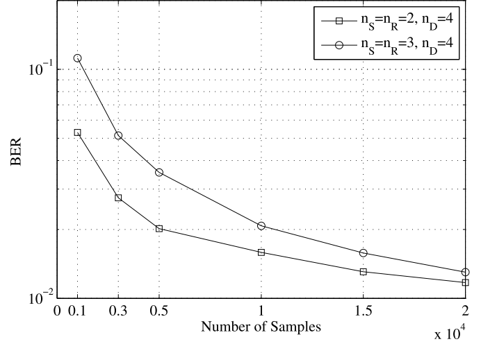
Fig. 2. Example 1: BER versus number of samples for various n_S and n_R with \text{SNR}_{s-r} = \text{SNR}_{r-d} = 20 dB and n_D = 4 .
