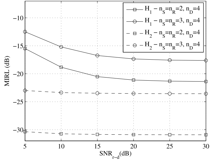
Fig. 4. Example 2: MIRL versus \text{SNR}_{r-d} for various n_S and n_R with \text{SNR}_{s-r} = 20 dB and n_D = 4 .
