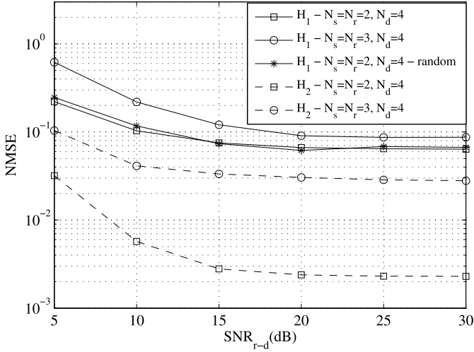
Fig. 5. Example 3: normalized MSE versus \text{SNR}_{r-d} for various n_s and n_r with \text{SNR}_{s-r} = 20 dB and n_D = 4 .
