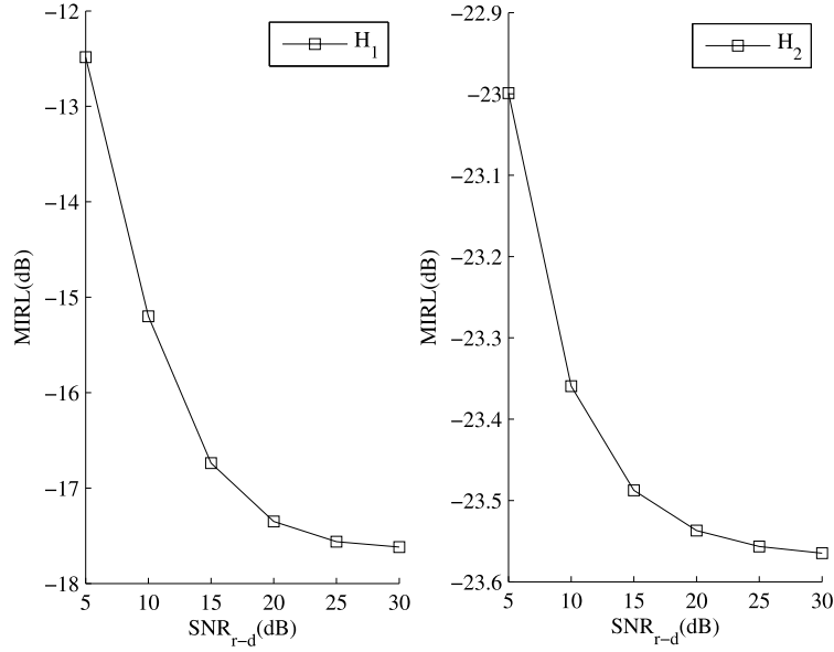
Fig. 3. Example 2: MIRL versus \text{SNR}_{r-d} for n_S = n_R = 3 , n_D = 4 , and \text{SNR}_{s-r} = 20 dB.
