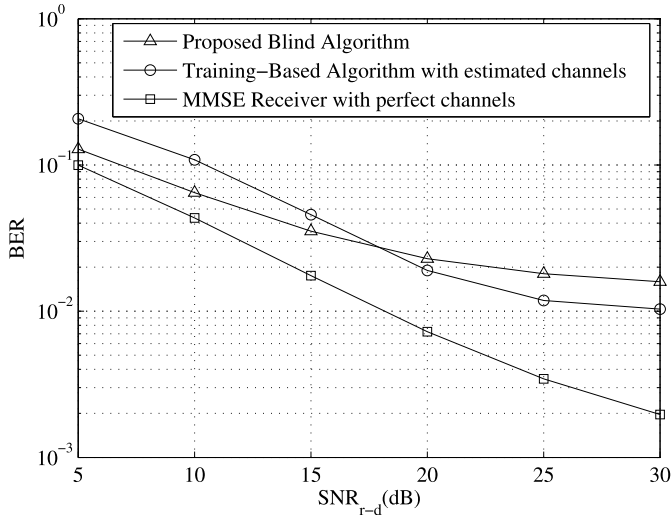
Fig. 8. Example 4: BER versus \text{SNR}_{r-d} for n_S = n_R = 2 and n_D = 4 with \text{SNR}_{S-r} = 20 dB.
