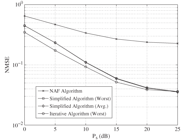
Fig. 2. Example 1: Normalized MSE versus P_s . K = 2, L = 3, M = 2, N_s = 2, N_1 = 8, N_2 = 4, N_d = 8, P_r = 20 dB.
